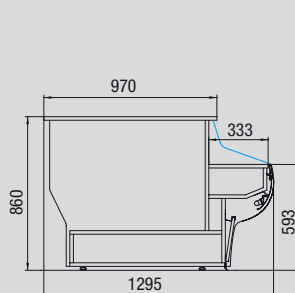
Prolunga - Extension Counter
